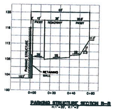
GRADING SECTIONS SCALE AS NOTED
